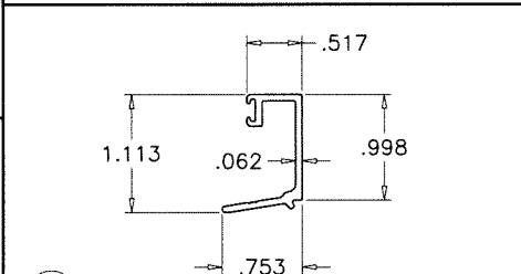
10 GLAZING BEAD (5/16" LAM. GLASS)
