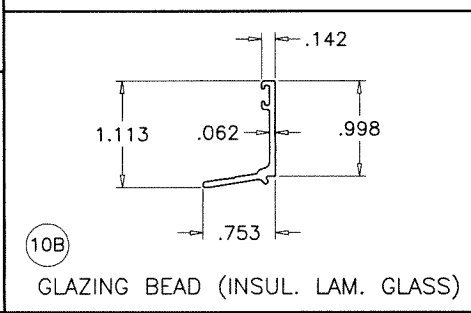
10A GLAZING BEAD (7/16" LAM. GLASS)
