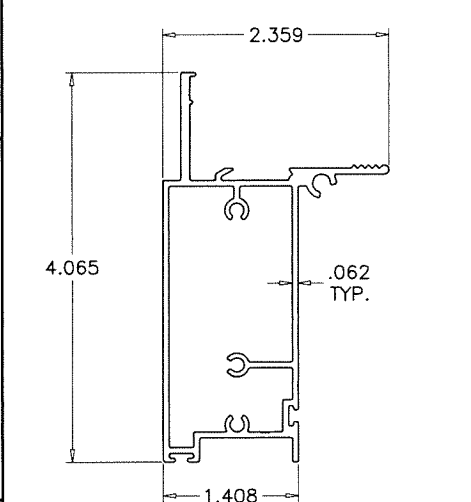
6 BOTTOM RAIL
