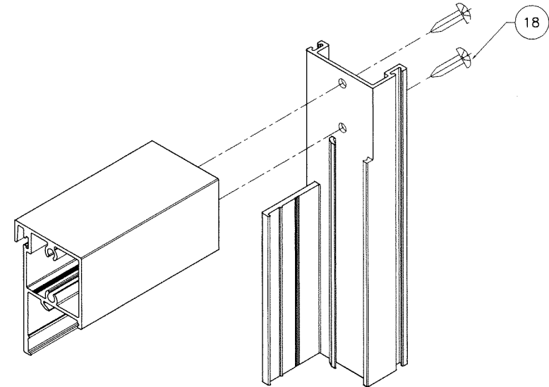
VENT TOP CORNER
